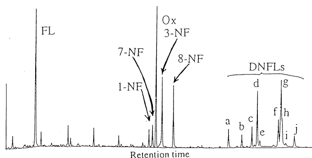
Figure 1. Typical GC-FID chromatogram of an extract from the sample supported on Fe 2 O 3 after 4 h exposure to 10 ppm NO 2 -5 ppm O 3 -O 2 in the dark.
