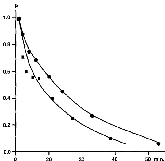
Fig. 1. Disappearance of 1 (squares) and 3 (circles) as monitored by the normalized intensities ( P ) of their ^1H -NMR signals
