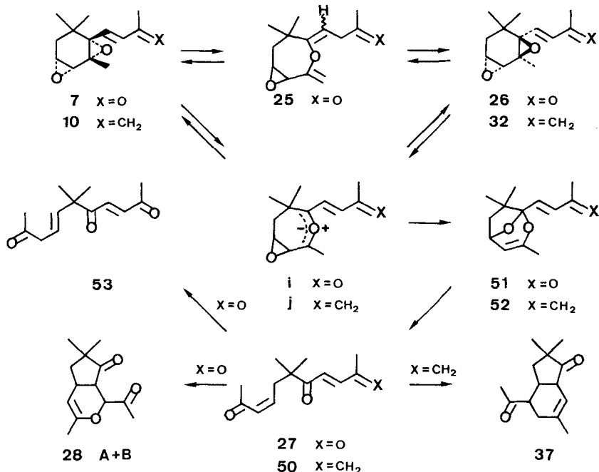
Scheme 7
