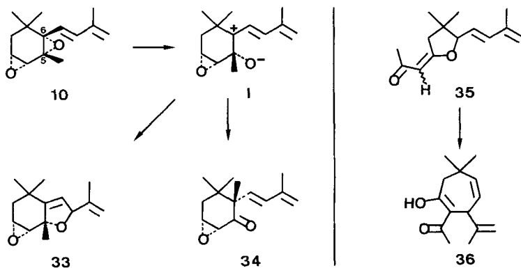
Scheme 8
