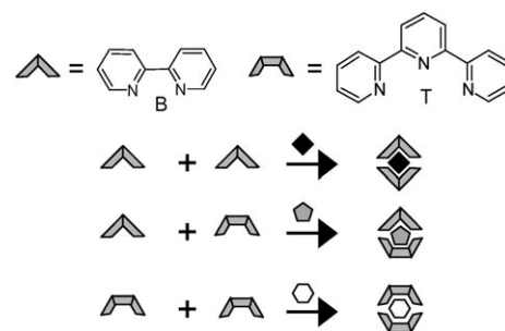
Figure 1. Coordination patterns and corresponding pair-coding with bidentate (B; bipyridine) and tridentate (T; terpyridine) ligand subunits; tetra- (e.g., \text{Cu}^{\text{I}} ), penta- (e.g., \text{Cu}^{\text{II}} ), and hexacoordinating (e.g., \text{Zn}^{\text{II}} , \text{Fe}^{\text{II}} ) metal ions are represented for simplicity by a square, a pentagon and a hexagon, respectively.
