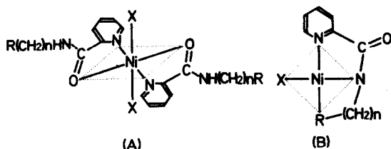
Figure 1. Proposed structures for (A) [\text{NiX}_2(\text{LH})_2]^{p+} and (B) [\text{NiXL}] \cdot \text{mH}_2\text{O} .
