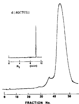
FIGURE 1 : DEAE Sephadex A25 Chromatography [linear gradient of triethylammonium bicarbonate (pH 7.5) from 0.001-1.0 M] of d[AGCTCG]. Inset: h.p.l.c. (Jones APEX ODS column) of main peak.
