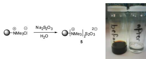
Scheme 3 A resin for scavenging iodine.
