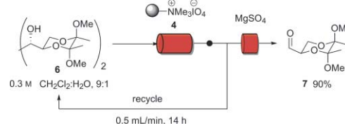
Scheme 6 Continuous flow synthesis of BDA-protected aldehyde 7 .
