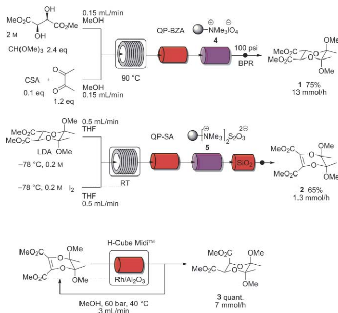
Scheme 1 Flow syntheses of butane-2,3-diacetal tartrates using the Uniqsis FlowSyn.
