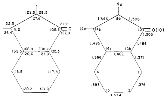
Figure 6. Bond distances and angles in the second indeno group with the planar five-membered ring.
