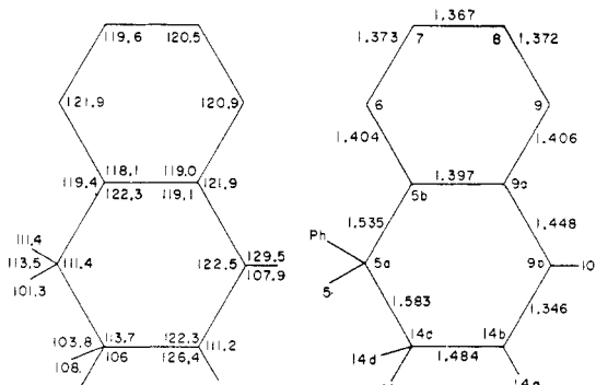
Figure 7. Bond distances and angles in the benz group and central six-membered ring.
