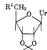
IIIa, R 1 = OH b, R 1 = I
