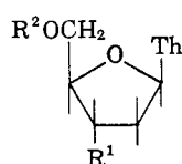
IVa, R 1 = OH, R 2 = acetyl b, R 1 = I, R 2 = acetyl c, R 1 = I, R 2 = H d, R 1 = OH, R 2 = p -nitrobenzoyl e, R 1 = I, R 2 = p -nitrobenzoyl
