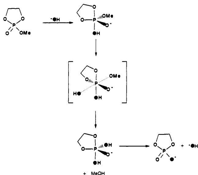
Scheme IX
