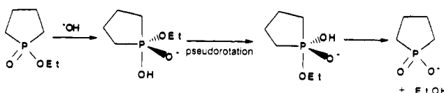
Scheme VIII
