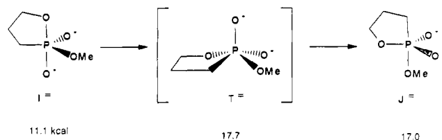
Scheme VII
