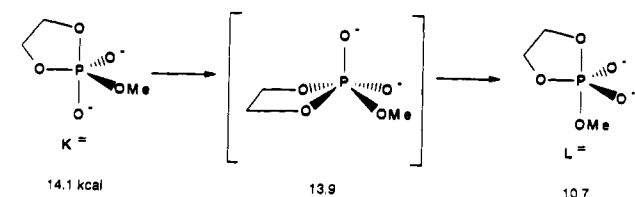
Scheme VIII
