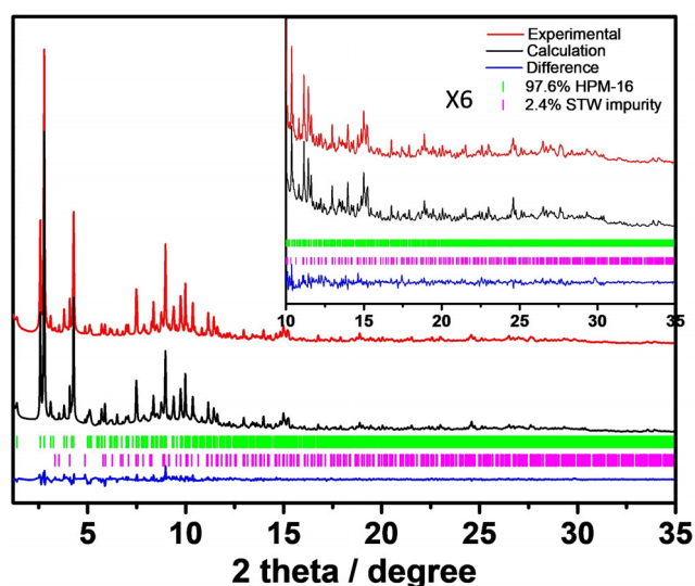
Figure 1. Rietveld refinement plot ( \lambda=0.618668 Å) for as-made HPM-16 (containing a small, < 3%, STW impurity, see SI). Red: experimental, black: calculated, blue: difference. Vertical bars are allowed reflections for HPM-16 (green) and STW (purple). CCDC NO. 2097880 and 2097878 for as-made and calcined HPM-16, respectively.
