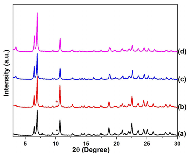
Figure 4. Powder X-ray diffraction patterns of HPM-16: a) as-made, b) after ozone treatment, c) after final run of degermanation, and d) calcined at 800^\circ\text{C} after final run of degermanation. * marks a trace impurity of STW in the as-made and ozone treated samples (a,b). This disappears during the degermanation treatment (c,d).
