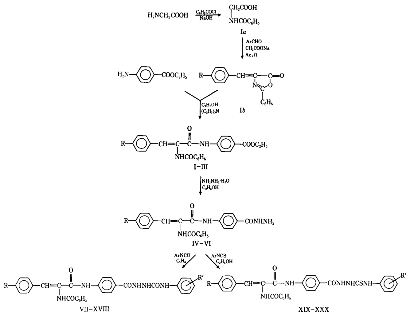
Scheme 1
