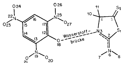
Fig. 1. 2-Dimethylamino-4,4-dimethyl-2-thiazolin-5-thion-Pikrat ( 17-Pikrat )
