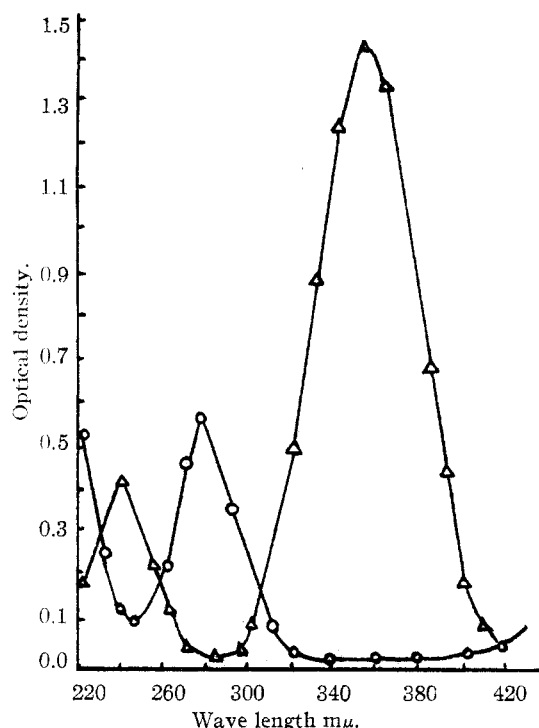
Fig. 1.—Absorption spectra of O, 2,5-dicarboxypyrazine; Δ, 2,5-diaminopyrazine.
