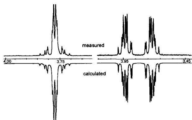
Fig. 7. ^1\text{H} NMR (360 MHz) (ppm): methylene region of (a) 3 at 311 K and (b) 4 at 340 K.
