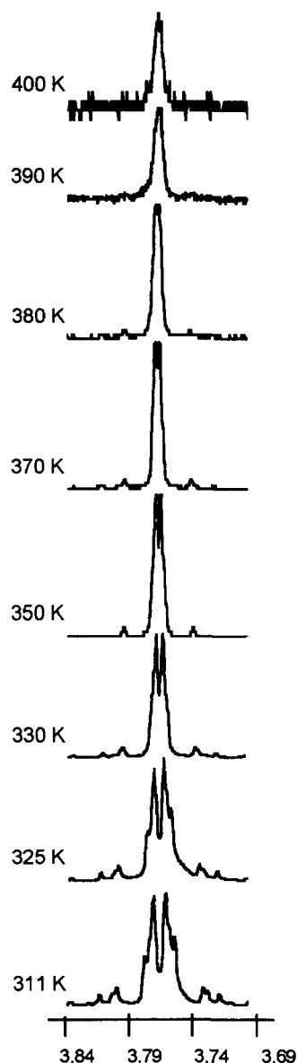
Fig. 8. Temperature dependent ^1\text{H} NMR (360 MHz) (ppm) of the methylene region of 3 .
