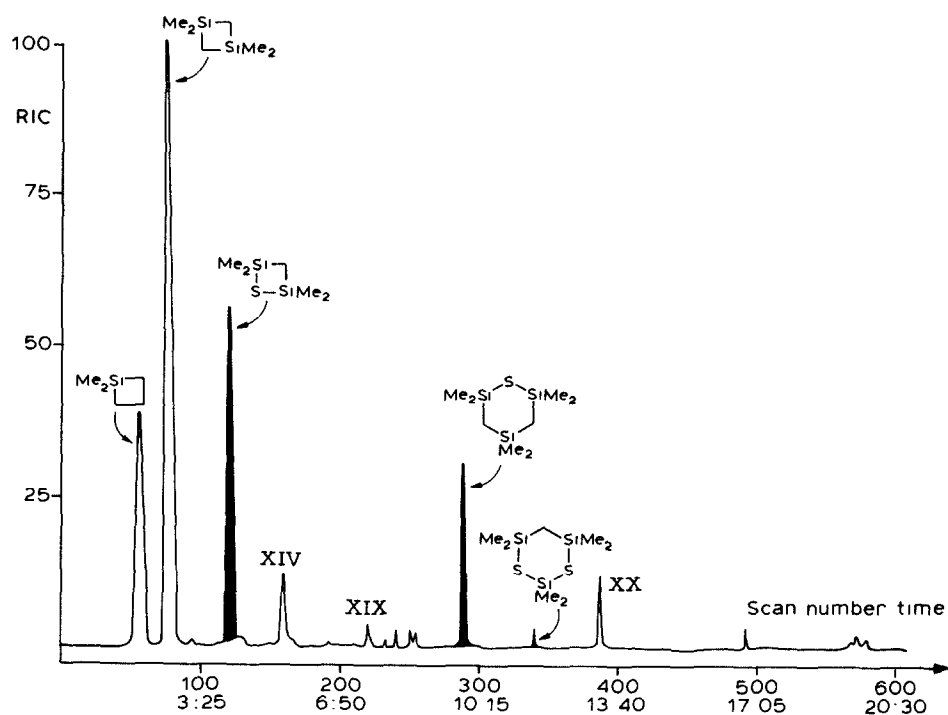
Fig. 4. Chromatogram of the copyrolysis products of I and III.
