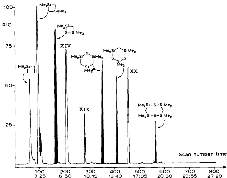
Fig. 1. Chromatogram of the copyrolysis products of I and II (5.4/1 mixture), showing the reconstructed ion current (RIC) against scan number (100,200...) and scan time (min:s).
