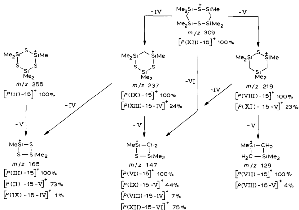
SCHEME 3. Fragmentation of [P-15]^+ ions in mass spectra of compounds II, VIII, IX and XII.
