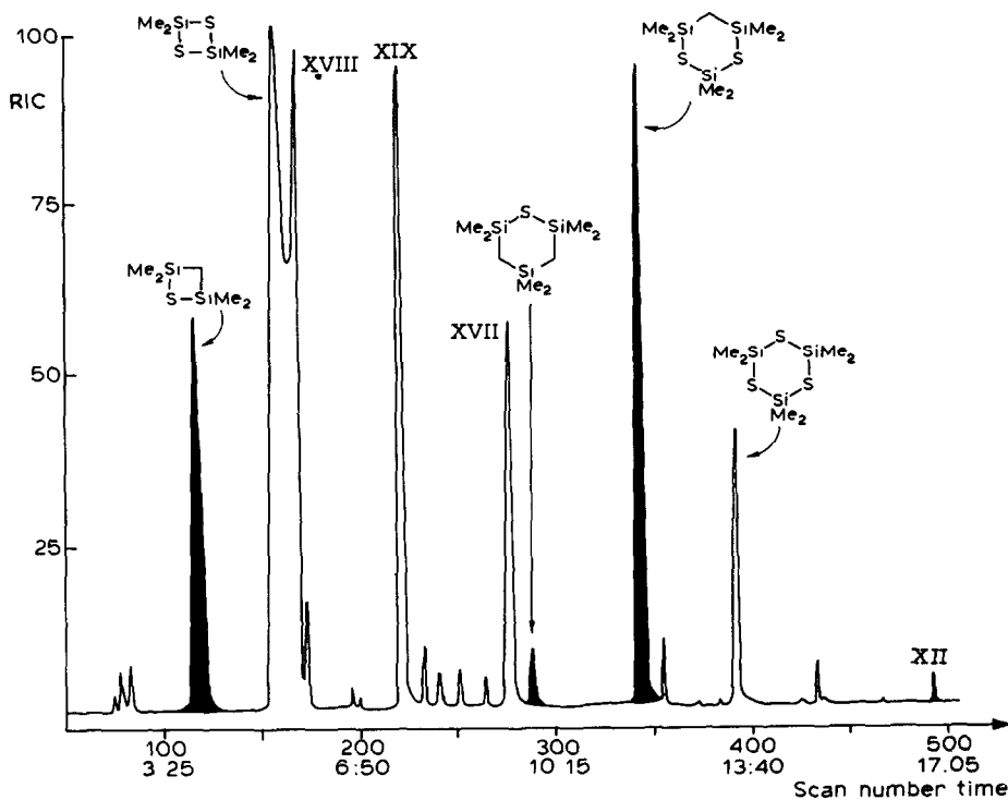
Fig. 2. Chromatogram of the copyrolysis products of I and II (1/1 mixture).
