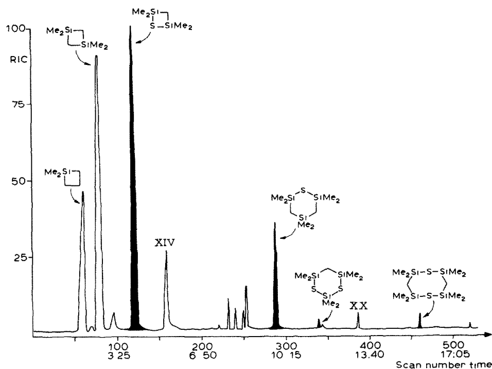
Fig. 6. Chromatogram of the copolylysis products of I and X.
