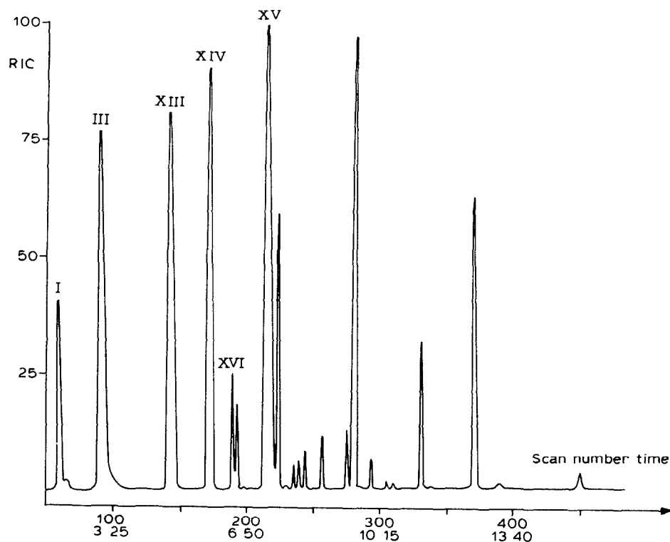
Fig. 3. Chromatogram of the hydrolysed copyrolysis products of I and II.
