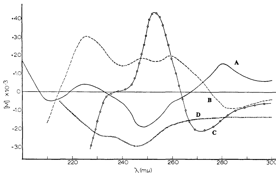
Figure 8. ORD curves: A, 6-chloro-9-(3',4'-di- O -acetyl-2'-deoxy- \alpha -D-ribofuranosyl)purine (V) (—); B, 6-chloro-9-(3',4'-di- O -acetyl-2'-deoxy- \beta -D-ribofuranosyl)purine (III) (---); C, 6-amino-9-(2'-deoxy- \alpha -D-ribofuranosyl)purine (VIII) (o-o-o); D, 6-amino-9-(2'-deoxy- \beta -D-ribofuranosyl)purine (VII) (••••).
