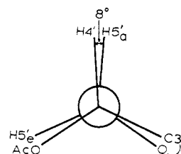
Figure 7. Newman projection of the carbohydrate moiety of 6-chloro-9-(3',4'-di-O-acetyl-2'-deoxy- \alpha -D-ribosepyranosyl)purine (V) as viewed down the C4'-C5' bond.
