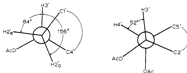
Figure 6. Newman projections of the carbohydrate moiety of 6-chloro-9-(3',4'-di-O-acetyl-2'-deoxy- \alpha -D-ribosepyranosyl)purine (V) as viewed down the C2'-C3' bond and the C3'-C4' bond.
