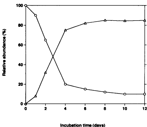
Fig. 1. Time-course for the biotransformation of 1 by G. cingulata . \circ = ( \pm )- cis -Nerolidol ( 1 ); \triangle = ( Z )-3,7,11-trimethyl-1,6-dodecadien-3,10,11-triol ( 2 ).
