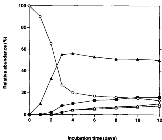
Fig. 2. Time-course for the biotransformation of 3 by G. cingulata . ○ = Nerylacetone (3); ▲ = (Z)-9,10-dihydroxy-6,10-dimethyl-5-undecen-diol-2-one (4); ■ = (Z)-6,10-dimethyl-5,9-undecadien-2-ol (5); △ = (Z)-10-hydroxy-6,10-dimethyl-5-undecen-2-one (6); □ = (Z)-6,10-dimethyl-5-undecen-2,9,10-triol (7).
