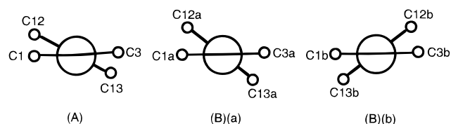
Figure 7. Newman projections of parts of molecules of (A) and (B), looking in the C(2)–C(11) direction.
