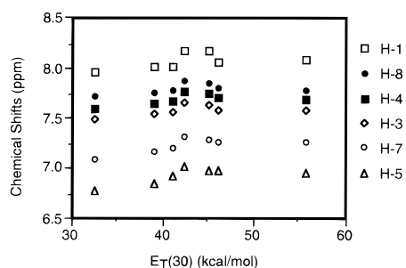
Figure 1. ^1\text{H} NMR chemical shifts for naphthalene protons in DDNP vs solvent E_T(30) values. 25 Proton assignments were made from single proton decoupling experiments.
