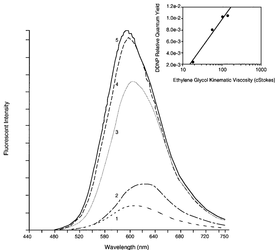
Figure 3. Corrected room temperature fluorescence emission spectra of DDNP in MeOH (1, 0.695 cSt), ethylene glycol (2, 18 cSt), and neat polyethylene glycol mixture of different viscosities (3), PEG200, 58 cSt; (4), PEG400, 105 cSt; and (5), PEG 600, 140 cSt. Excitation = 420 nm. Inset shows the relationship between quantum yield and viscosity in the polyethylene glycol series. \log_{10} curve fit R^2 = 0.982 . Note: changes in fluorescence emission wavelength are probably due to changes in solvent polarities.
