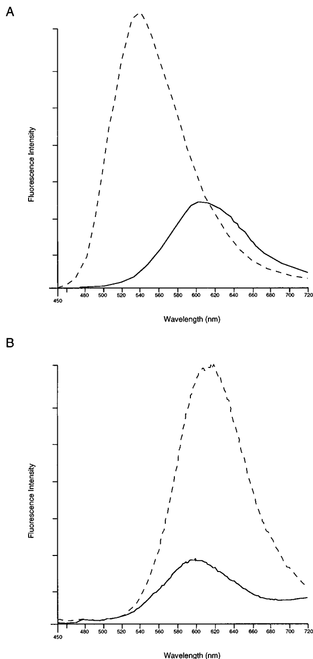
Figure 5. A. Molecule fluorescence emission spectra of DDNP in glycerol at room temperature (—) and glycerol at -50\% (---); B, in methanol at room temperature (—) and methanol at -50^\circ (---). Excitation at 460 nm.
