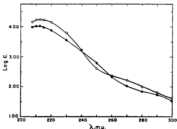
Fig. 1.—Absorption spectra: O—O, obacunone in methanol; ●—●, obacunoic acid in ethanol. Although the region below 220 mμ is beyond the most accurate range of the instrument, the curves are certainly at least qualitatively correct.
