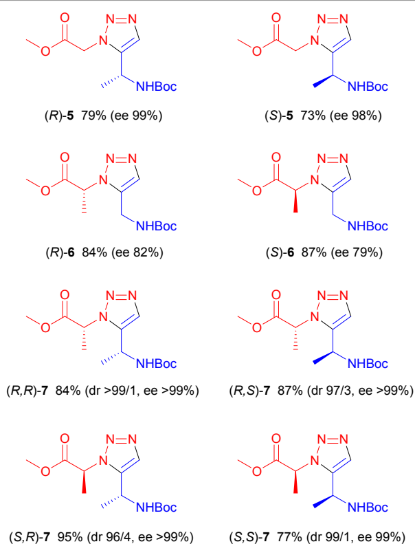
Fig. 2 Chiral 1,5-substituted triazoles prepared via RuAAC. See experimental section for method used.
