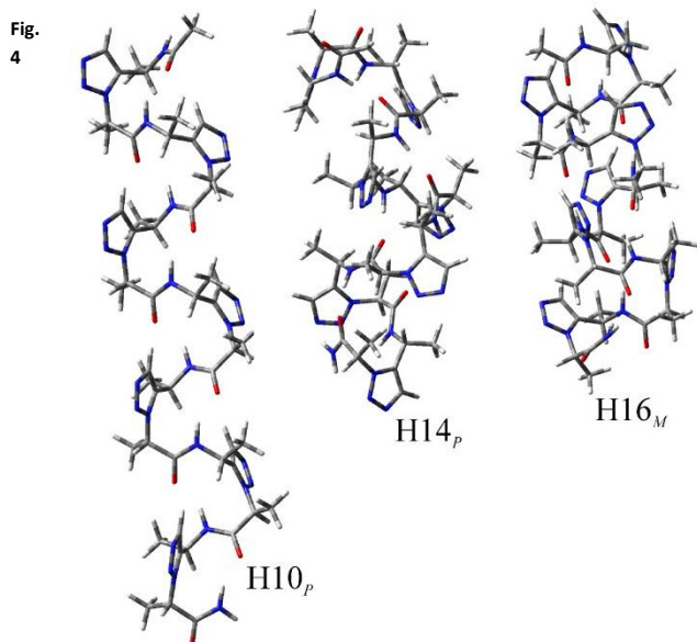
Fig. 4 The three most stable conformation of ( S,R )-7 heptahomooligomer. Calculations were performed at the \omega B97X-D/6-31+G(d,p) // \omega B97X-D/6-31G(d) level of theory.
