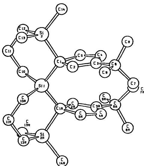
Fig. 2. Crystal structure of ligand 9b .
