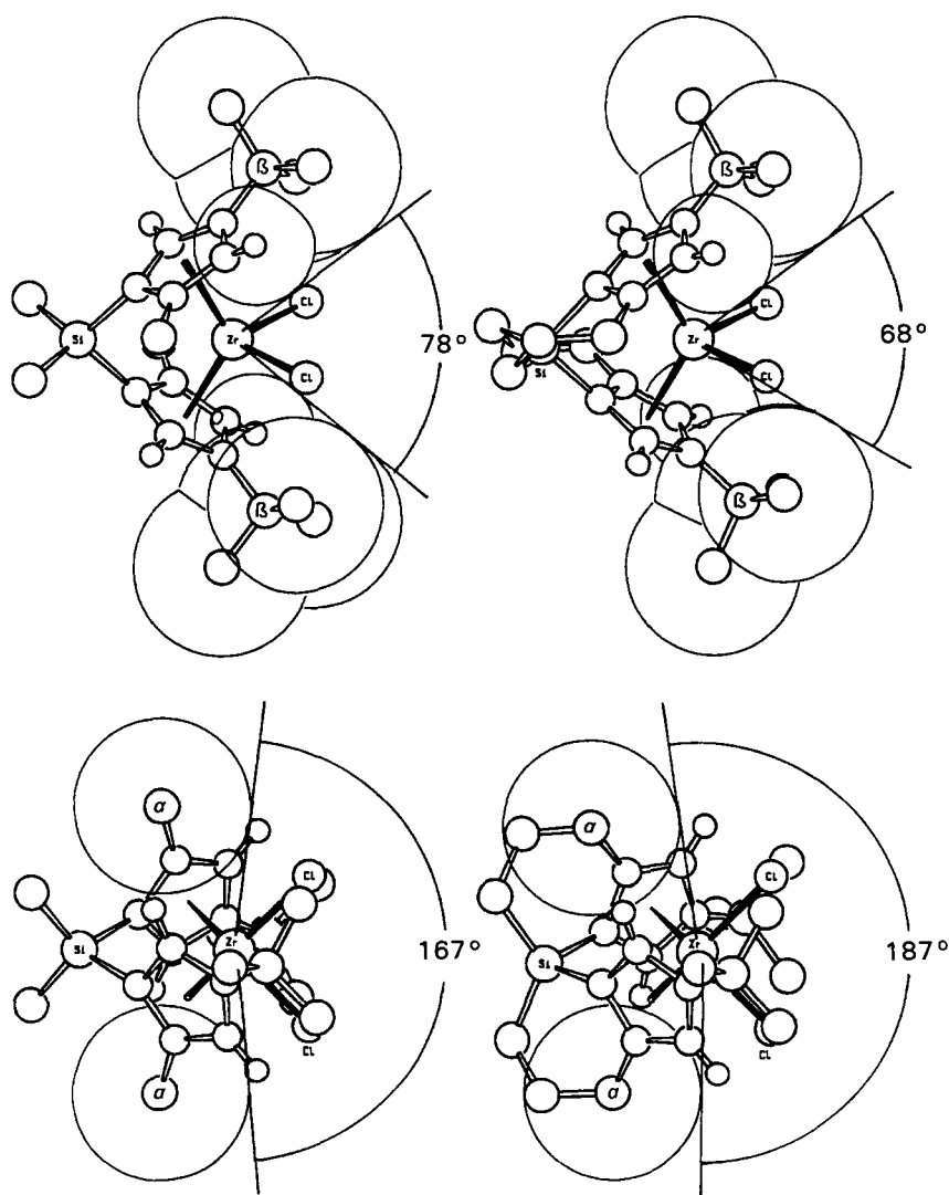
Fig. 3. Gap aperture (top) and lateral extension angles (bottom) for the Me 2 Si-bridged complex 2d (left) and the spiro-silane-bridged complex 3d (right, cf. Appendix A).
