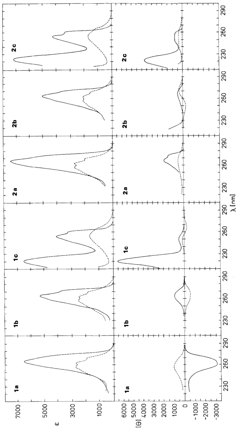
Fig. 1. UV- and CD-spectra of the 2-, 3- and 4-(1-methylpropyl)- (1a, b, c) and of 2-, 3- and 4-(2-methylbutyl)pyridines (2a, b, c): (---) alkyl pyridine in hexane; (—) alkyl pyridine and TFA in hexane, molar ratio (TFA)/(alkyl pyridine) = 10
