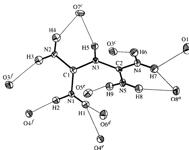
Fig. 1. The biguanidium cation in (\text{BIGH}_2)(\text{ClO}_4)_2 showing the hydrogen bonds. Displacement ellipsoids are shown at the 50% probability level [symmetry codes: (a) -x, 1-y, -z ; (b) 1-x, 1-y, -z ; (c) 1+x, y, z ; (d) 1+x, 1+y, z ; (e) x, 1+y, z ; (f) -x, 1-y, 1-z ].
