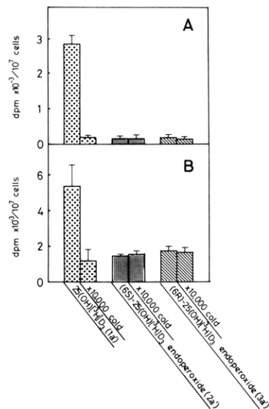
Figure 1. Incorporation of 25-(OH)[ ^3H ] D_3 endoperoxides ( 2a' and 3a' ) and 25-(OH)[ ^3H ] D_3 ( 1a' ) into the cytosol (A) and chromatin (B) fractions of HL-60 cells. HL-60 cells were incubated with 3.2 nM 25-(OH)[ ^3H ] D_3 endoperoxides or 25-(OH)[ ^3H ] D_3 in the presence or absence of a 10 000-fold excess of the respective compounds for 1 h at 37 °C under 5% CO_2 in air. After incubation, cells were homogenized and fractionated. The cytosol fraction was treated with hydroxylapatite to separate protein-bound 25-(OH)[ ^3H ] D_3 endoperoxides or 25-(OH)[ ^3H ] D_3 from the respective free radioisotopes: \square , 25-(OH)[ ^3H ] D_3 ( 1a' ); \square , (6 S )-25-(OH)[ ^3H ] D_3 endoperoxide ( 2a' ); \square , (6 R )-25-(OH)[ ^3H ] D_3 endoperoxide ( 3a' ).
