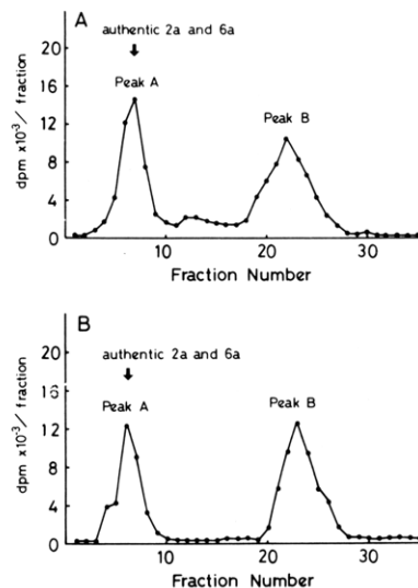
Figure 2. Sephadex LH-20 chromatographic profiles of extracts of culture medium with (A) or without (B) HL-60 cells after incubation with (6 S )-25-(OH)[ ^3H ] D_3 endoperoxide ( 2a' ) for 3 days. (6 S )-25-(OH)[ ^3H ] D_3 endoperoxide (3.0 nM) was incubated with culture medium with or without HL-60 cells at 37 °C under 5% CO_2 in air for 3 days. The extract was chromatographed on Sephadex LH-20 column (1.2 \times 25 cm) with chloroform-hexane (3:1), and 4-mL fractions were collected. The arrow indicates the elution position of authentic (6 S )-25-(OH) D_3 endoperoxide ( 2a ) and 25-hydroxy-6,19-epoxyvitamin D_3 ( 6a ).
