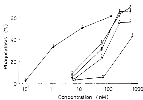
Figure 5. Comparison of the dose-response effects of various derivatives of vitamin D 3 in inducing phagocytic activity in HL-60 cells incubated for 3 days: ●, 1 \alpha ,25-(OH) 2 D 3 ; ◇, (6S)-19,25-dihydroxy-6,19-dihydro-6,19-epoxyvitamin D 3 ( 4a ); ◆, 25-hydroxy-6,19-epoxyvitamin D 3 ( 6a ); □, (6S)-25-(OH)D 3 endoperoxide ( 2a ); ▲, 25-(OH)D 3 ( 1a ). The control value was 2.9 \pm 0.5%. Points are means \pm SEM (represented by the bars) of six replicates.
