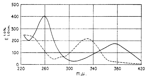
Fig. 2.—Ultraviolet absorption spectra of 2-amino-4-hydroxy-7-dibromomethylpteridine hydrobromide: —, 0.1 N sodium hydroxide; ---, 0.1 N hydrochloric acid.
