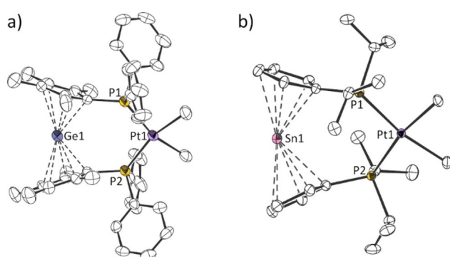
Figure 13. Molecular structures of (a) 2-PtMe 2 and (b) 3b-PtMe 2 in the crystal (displacement ellipsoids at the 50% probability level; H atoms omitted). Selected bond lengths [pm] and angles [°]: 2-PtMe 2 : P1–Pt1 229.40(1), P2–Pt1 229.46(1), Cp cent –Ge1 219.77(1)/220.17(1); Cp cent –Ge1–Cp cent 162.993(2), P1–Pt1–P2 107.338(2); 3b-PtMe 2 : P1–Pt1 232.80(2), P2–Pt1 232.34(2), Cp cent –Sn1 237.30(2)/243.11(2); Cp cent –Sn1–Cp cent 149.810(4), P1–Pt1–P2 105.935(4).
