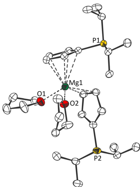
Figure 3. Molecular structure of 1b·(thf) 2 in the crystal (displacement ellipsoids at the 50% probability level; H atoms omitted). Selected bond lengths [pm]: Mg1–O1 208.14(1), Mg1–O2 206.17(2), Cp cent –Mg1 224.05(2).
