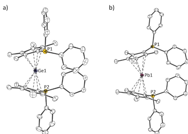
Figure 8. Molecular structures of (a) 2 and (b) 4 in the crystal (displacement ellipsoids at the 50% probability level; H atoms omitted). Selected bond lengths [pm] and angles [°]: 2 : Cp cent –Ge1 220.20(3)/222.33(3); Cp cent –Ge1–Cp cent 159.932(15); 4 : Cp cent –Pb1 247.82(2)/249.19(2); Cp cent –Pb1–Cp cent 150.575(11).
