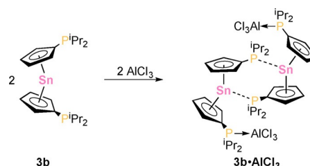
Scheme 8. Reaction of 3b with 1 equivalent of AlCl 3 .
