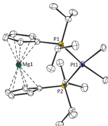
Figure 6. Molecular structure of 1b·PtMe 2 in the crystal (displacement ellipsoids at the 50% probability level; H atoms omitted). Selected bond lengths [pm] and angles [°]: P1–Pt1 231.19(4), P2–Pt1 232.73(4), Cp cent –Mg1 197.34(6)/198.57(6); Cp cent –Mg1–Cp cent 164.409(32), P1–Pt1–P2 105.129(13).
