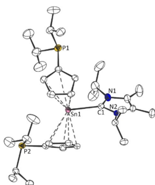
Figure 10. Molecular structure of 3b-NHC in the crystal (displacement ellipsoids at the 50% probability level, H atoms omitted). Selected bond lengths [ppm] and angles [°]: Sn1–C1 241.63(0), \text{Cp}^{\text{cent}}\text{--Sn1} 259.31(1)/264.86(1); \text{Cp}^{\text{cent}}\text{--Sn1--Cp}^{\text{cent}} 134.767(1).
