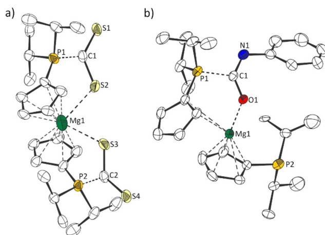
Figure 5. Molecular structure of (a) 1b·(CS 2 ) 2 and (b) 1b·PhNCO in the crystal (displacement ellipsoids at the 50% probability level; H atoms omitted). Selected bond lengths [pm] and angles [°]: 1b·(CS 2 ) 2 : Mg1–S2/S3 249.48(39), Cp cent –Mg1 215.39(8), P1–C1/P2–C2 183.71(124); Cp cent –Mg1–Cp cent 136.61(2); 1b·PhNCO : Mg1–O1 195.65(1), P1–C1 184.80(18), Cp cent –Mg1 218.16(8).
