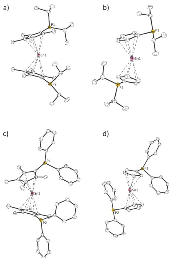
Figure 7. Molecular structures of (a) 3a , (b) 3b , (c) 3c , and (d) 3d in the crystal (displacement ellipsoids at the 50% probability level, H atoms omitted). Selected bond lengths [pm] and angles [°]: 3a : Cp cent –Sn1 237.67(1)/240.43(1); Cp cent –Sn1–Cp cent 156.147(3); 3b : Cp cent –Sn1 240.39(1)/242.21(1); Cp cent –Sn1–Cp cent 152.593(2); 3c : Cp cent –Sn1 240.93(1)/242.09(1); Cp cent –Sn1–Cp cent 152.753(3); 3d : Cp cent –Sn1 242.92(1)/242.93(1); Cp cent –Sn1–Cp cent 146.951(4).
