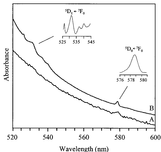
Figure 2. Electronic spectra of 1 as solid (A) and HOPr i solution (B). (The insert picture spectrum of the of the ^5D_1 \leftarrow ^7F_0 transition has been baseline corrected with a straight line.)
