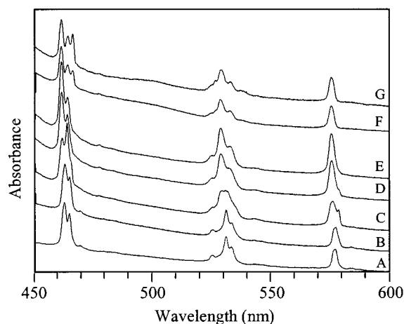
Figure 11. ^5D_2 \leftarrow ^7F_0 , ^5D_1 \leftarrow ^7F_0 , and ^5D_0 \leftarrow ^7F_0 transitions of \text{Eu}^{3+} in toluene/ \text{HOPr}^i (2:1) solutions of 2 (A); 2 and \text{Al}_4(\text{OPr}^i)_{12} (Eu/Al 1:3) after 24 h at room temperature (B), 30 min at 75 °C (C), 60 min at 75 °C (D), 80 min at 75 °C (E), 120 min at 75 °C (F); and 3 (G).
