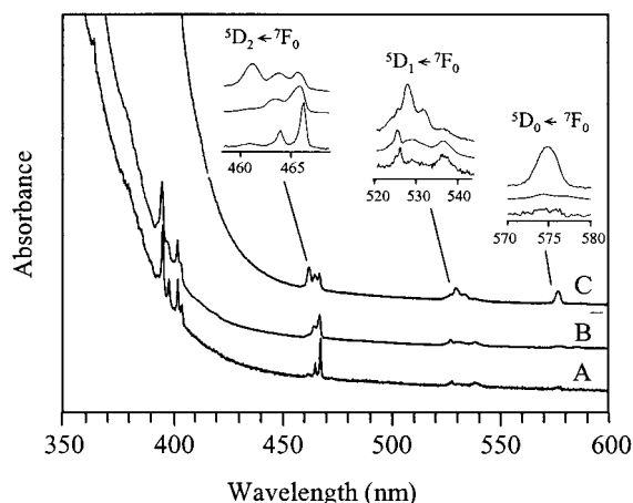
Figure 9. Electronic spectra of 3 as solid (A), hexane solution (B), and hexane/HOPr i (1:1) solution (C).
