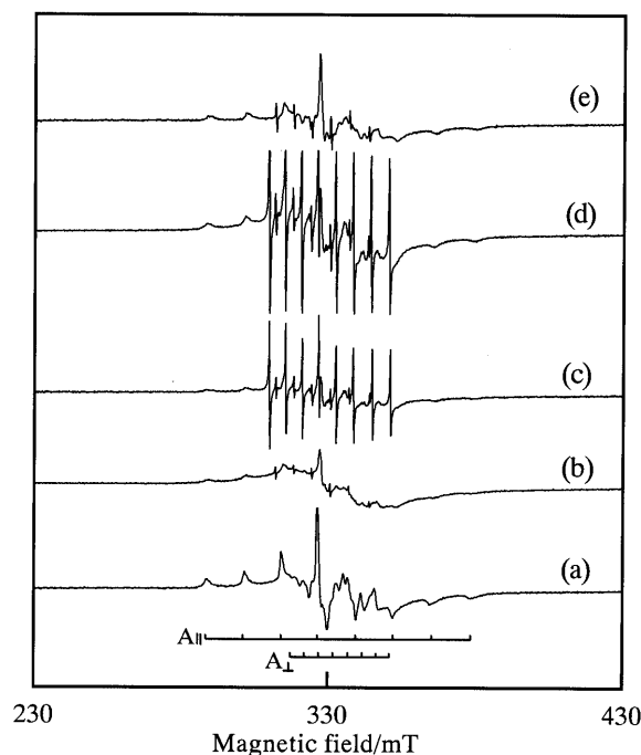
Figure 1. ESR spectra of V(1.0)/MgO-100A catalysts treated under various conditions.
