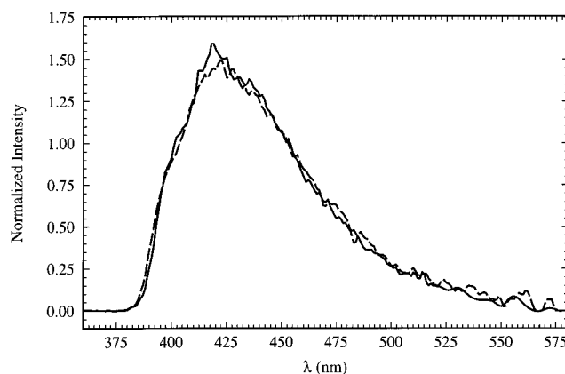
Figure 9. c -APE fluorescence spectra based on three-spectra sets for \lambda_{\text{exc}} = 374 nm (—, [\text{c-APE}] = 3.4 \times 10^{-5} M) and \lambda_{\text{exc}} = 402 nm (---, [\text{c-APE}] = 1.4 \times 10^{-4} M).
