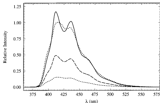
Figure 5. A typical set of fluorescence spectra of c -APE ( 1.4 \times 10^{-4} M) in Ar (—), air (---) and O 2 -saturated (···) toluene solution obtained for \lambda_{\text{exc}} = 390 nm. The spectrum for the O 2 -saturated solution is also shown multiplied by a factor of 6.64 (the area ratio). The spectra are corrected for background and self-absorption, but not for nonlinearity of instrumental response.
