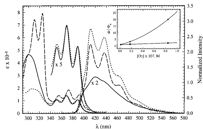
Figure 1. Absorption spectra of c -APE (—) and t -APE (---) and fluorescence excitation spectrum ( \lambda_{\text{em}} = 415 nm) of c -APE (· · ·) and contributions of ^1t\text{-APE}^* (— · —) and ^1c\text{-APE}^* ( \times 2 ) (—) emissions in c -APE fluorescence ( \lambda_{\text{exc}} = 366 nm) (· · ·) in toluene at 20 °C. All fluorescence spectra are corrected for nonlinearity in instrumental response. Inset: Global Stern–Volmer plots for the \text{O}_2 effect on resolved fluorescence areas of c -APE and t -APE B .
