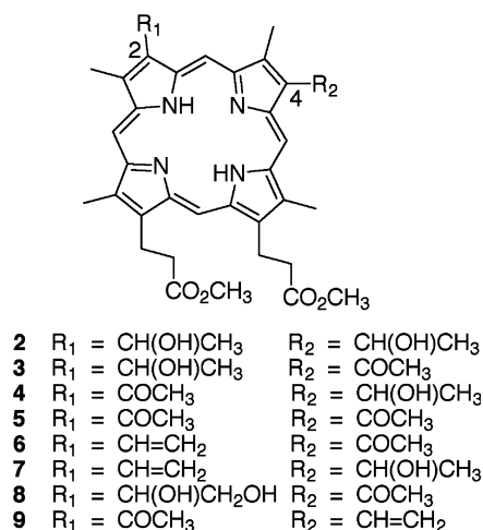
Fig. 1. Porphyrin monomers prepared regioselectively in preparation for ether-linked porphyrin dimers.
