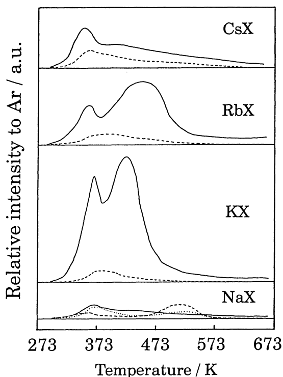
Fig. 1. TPD plots of CO 2 adsorbed on various zeolites; 13X •••, ion-exchanged ---, ion-added —.
