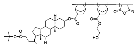
Figure 2. The chemical structure of poly(TBNC-co-HENC-co-MA).
