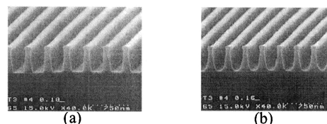
Figure 3. Scanning electron micrographs of 0.18 \mu\text{m} (a) and 0.16 \mu\text{m} (b) features with a thickness of 0.5 \mu\text{m} printed with poly(TBNC-co-HENC-co-MA) at a dose of 6 \text{mJ cm}^{-2} .
