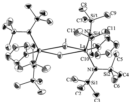
Fig. 1. Structure of iodo bis(bis(trimethylsilyl) lanthanum amide 3a .
