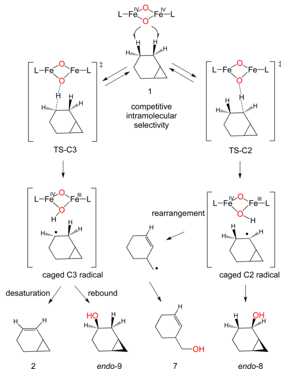
Figure 5. Mechanism of parallel, competitive desaturation, hydroxylation and rearrangement of norcaradiene ( 1 ) mediated by AlkB. The structure of the active species is modeled in analogy to compound Q of sMMO.
