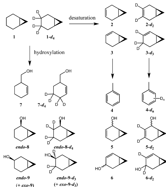
Scheme 1. Products from Norcarane Hydroxylation and Desaturation Mediated by AlkB
