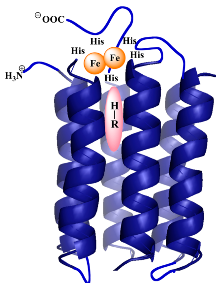
Figure 1. Depiction of the structure of AlkB showing six trans-membrane helices, the histidine-rich diiron active site and a long, inter-helix substrate binding channel from the homology model of van Beilen et al. 14
