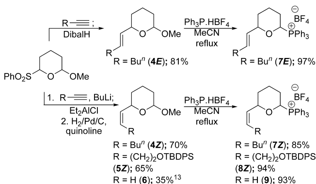
Scheme 1. Synthesis of Enol Ether Precursors
