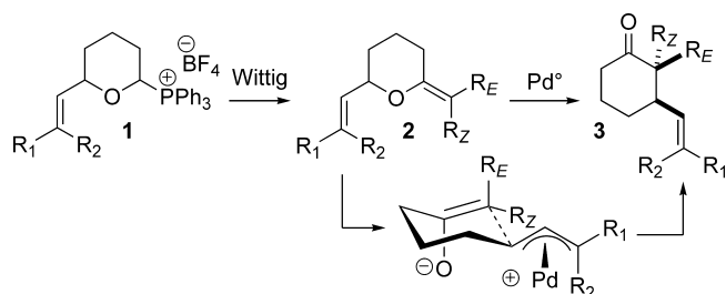
Figure 1. Pd-catalyzed O-to-C rearrangement.
