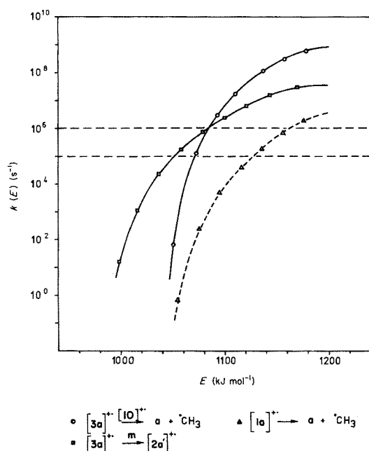
Figure 4. Calculated rate constants k(E) vs potential energy for the reactions [3a]^{+\bullet} \rightarrow a + CH_3 , [3a]^{+\bullet} \rightarrow [2a]^{+\bullet} and [1a]^{+\bullet} \rightarrow a + CH_3 .
