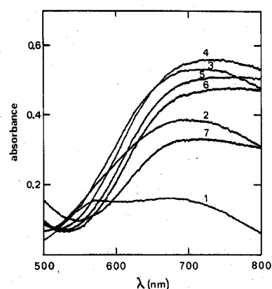
Figure 1. Visible spectra of 5.63 \times 10^{-3} \text{ M Cu}(\text{hfac})_2 in the presence of various amounts of ligand I in \text{CCl}_4 at 20 °C. The ligand:metal ratios for the successive scans are (1) 0.0, (2) 0.25, (3) 0.50, (4) 0.75, (5) 1.0, (6) 1.1, and (7) 2.0.
