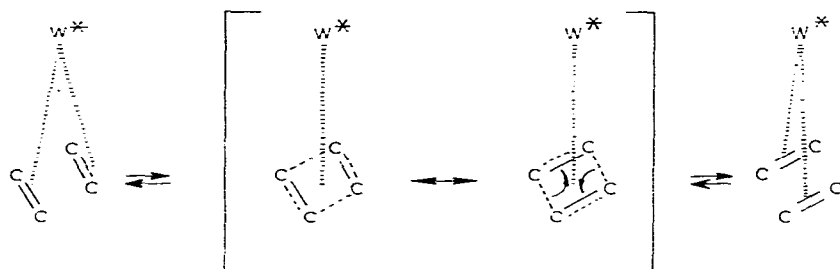
Fig. 6. 4-centre disproportionation mechanism.
