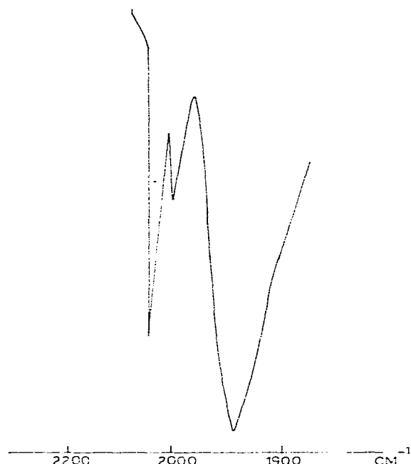
Fig. 2. IR spectrum (CO region) of a \text{Si-O-Ge[W(CO)}_3\text{Cp]}_3 type catalyst.
