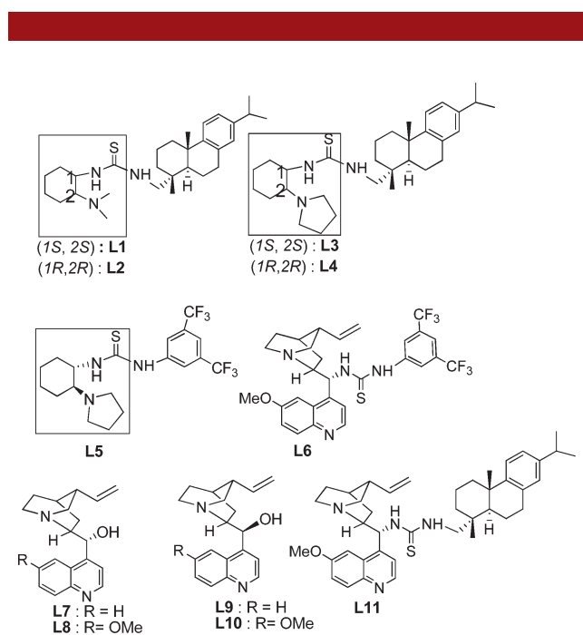
Figure 1. Organocatalysts used in this study.
