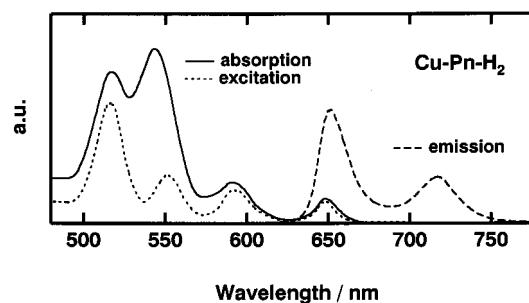
Figure 4. Fluorescence and its excitation spectra of Cu–Pn–H 2 together with the absorption spectrum of the Q-band in toluene.
