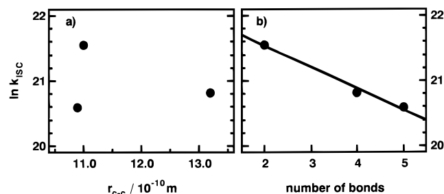
Figure 6. Semilogarithmic plots of k_{isc} versus (a) the center-to-center distance, r_{c-c} , which is calculated on MM2 and (b) number of bonds. The diameter of the circles in the figure indicates the size of experimental errors.
