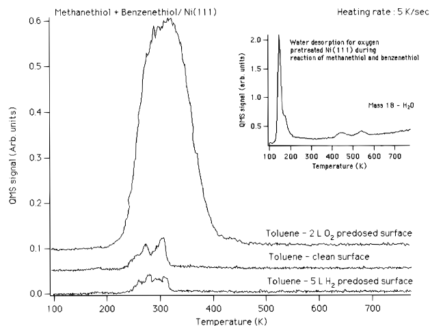
Figure 3. Thermal desorption spectra of toluene desorption from the Ni(111) surface predosed with oxygen, hydrogen, and a clean surface followed by approximately half-saturation coverages each of methanethiol and benzenethiol. Inset shows water desorption prior to toluene formation for the oxygen-predosed case.
