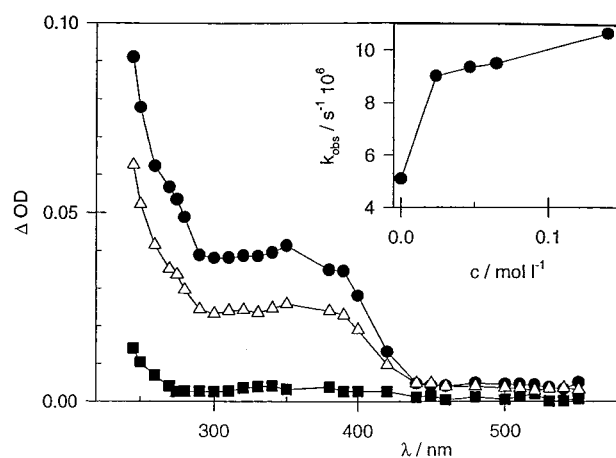
Figure 3. Optical absorption spectra taken after 266 nm flash photolysis of a solution of 0.1 M cyclohexanone in acetonitrile: (●) 30 ns, (△) 100 ns, and (■) 800 ns after the flash. The two absorption bands are assigned to the cyclohexanone triplet. The inset gives the Stern–Volmer plot due to reaction 12, i.e., the acceleration of the triplet decay in the presence of different concentrations of 1 .
