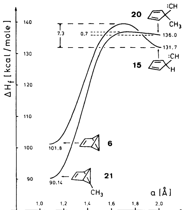
Fig. 3. Computed barriers (MINDO/3) for the linear cheletropic ring closure of carbenes 15 and 20 to the benzvalenes 6 and 21
