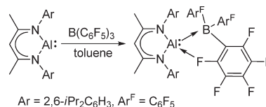
Scheme 4. Preparation of 5
