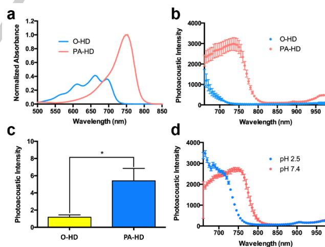
Figure 1. a) Absorbance and b) PA spectra of O-HD and PA-HD at pH 7.4 (1:1 v/v PBS:EtOH). Dye concentration was 25 \mu\text{M} for each dye (Each point represents Mean \pm SD, n = 3 ). c) Normalized photoacoustic intensity of O-HD and PA-HD in a tissue phantom containing 60% milk to mimic scattering effects in dense tissue. [PA-HD] = 0.5 \mu\text{M} (Mean \pm SD, n = 3 ). Statistical analysis was performed using two-tailed Student's t-test ( \alpha = 0.05 ), *: p < 0.05 . d) Photoacoustic spectra of PA-HD at pH 2.5 and 7.4 (Each point represents Mean \pm SD, n = 3 ).
