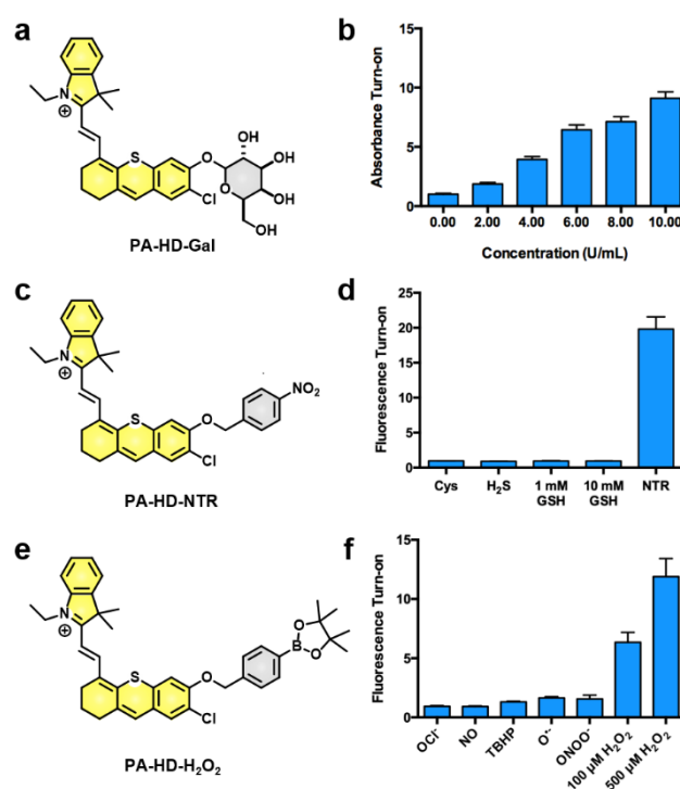
Figure 3. a) Chemical structure of PA-HD-Gal. b) Dose-dependent response of 5 \mu\text{M} PA-HD-Gal after 1 h to 0, 2, 4, 6, 8, or 10 U/mL of E. Coli beta-galactosidase at pH 7.4 (9:1 v/v PBS:MeCN) (Mean \pm SD, n = 5 ). c) Chemical structure of PA-HD-NTR. d) Response of 2 \mu\text{M} PA-HD-NTR to biologically relevant thiols (Cys and \text{H}_2\text{S} 100 \mu\text{M} ) and GSH at 1 mM and 10 mM for 15 min at pH 7.4 (9:1 v/v PBS:MeCN) (Mean \pm SD, n = 3 ). Complete activation mediated by 2 U/mL E. coli nitroreductase. e) Chemical structure of PA-HD- \text{H}_2\text{O}_2 . f) Response of 2 \mu\text{M} PA-HD- \text{H}_2\text{O}_2 to \text{OCl}^- , NO, TBHP, \text{O}_2^- , \text{ONOO}^- ( 100 \mu\text{M} ) and \text{H}_2\text{O}_2 ( 100 \mu\text{M} and 500 \mu\text{M} ) for 1 h at pH 7.4 (9:1 v/v PBS:MeCN) (Mean \pm SD, n = 3 ).
