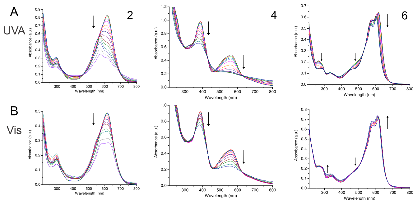
Figure 5. UV-visible absorption spectra of diazido complexes 2 , 4 and 6 after irradiation with (A) UVA and (B) visible white light, over 120 min in dioxane.
