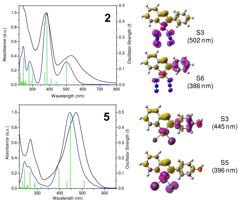
Figure 2. Left, normalized absorption spectra for azido complex 2 and chlorido complex 5 in methanol (black) and their corresponding TD-DFT spectra (blue). Calculated singlet electronic transitions are shown as green vertical bars with heights equal to their oscillator strength. Right, EDDMs of selected low-energy singlet electronic transitions for each complex. Electron density migrates from magenta to yellow areas.
