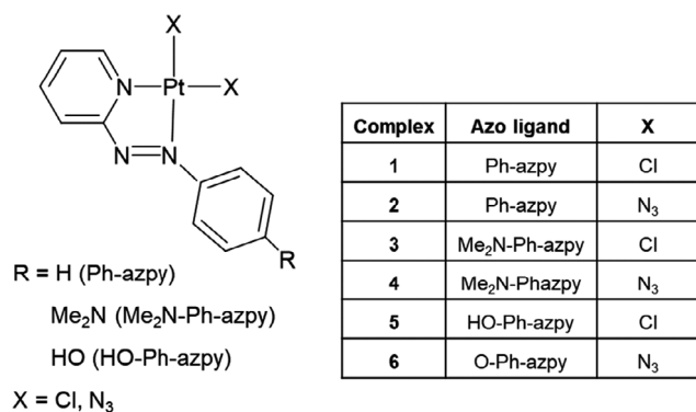
Figure 1. Structures of the Pt(II) azopyridine complexes studied in this work.
