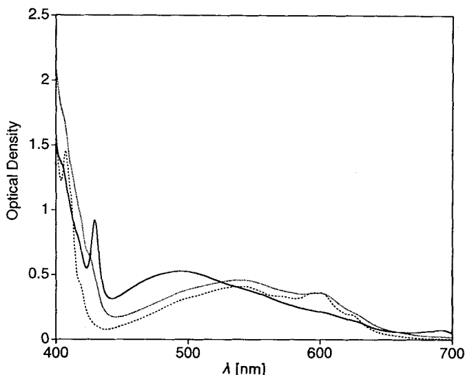
Fig. 6. Electronic-absorption spectra recorded in toluene ( T = 293\text{ K} , d = 1\text{ cm} ) of the mixture of (ethoxycarbonyl)methylene-bridged fullerenes 1a–3a with the relative intensity ratio 1:1:3 (·····, c undetermined), of pure isomer 1a (—, c = 4.13 \times 10^{-4}\text{ mol l}^{-1} ), and of C_{60} (-----, c = 5.11 \times 10^{-4}\text{ mol l}^{-1} )
