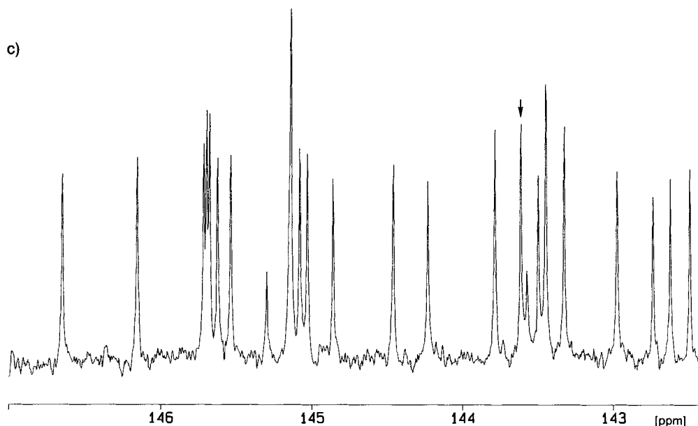
Fig. 4. 125.6-MHz ^{13}\text{C} -NMR Spectra recorded in \text{CS}_2 with (\text{D}_6) acetone as internal lock of a) the mixture of (ethoxycarbonyl)methylene-bridged fullerenes 1a , 2a , and 3a , b) pure isomer 1a , and c) the expanded 142–147-ppm region in the spectrum of pure 1a . The acetone resonances appear at 29.7 and 204.0 ppm and the solvent peak at 193.0. The arrow marks the resonance at 143.43 originating from a minor \text{C}_{60} impurity in the sample. T = Toluene.
