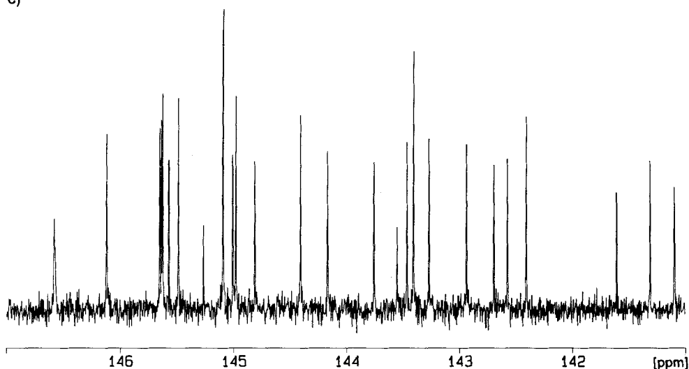
Fig. 5. 125.6-MHz ^{13}\text{C} -NMR Spectra recorded in \text{CS}_2 with (D_6) acetone as internal lock of a) the mixture of [(tert-butoxy)carbonyl]methylene-bridged fullerenes 1b , 2b , and 3b , b) pure isomer 1b , and c) the expanded 141–147-ppm region in the spectrum of pure 1b . The acetone resonances appear at 29.7 and 204.0 ppm and the solvent peak at 193.0. X in spectrum b): \text{Et}_2\text{O} . T = Toluene.
