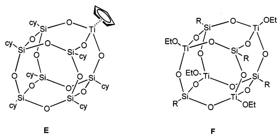
Chart 2. Cage-like titanasiloxanes.
