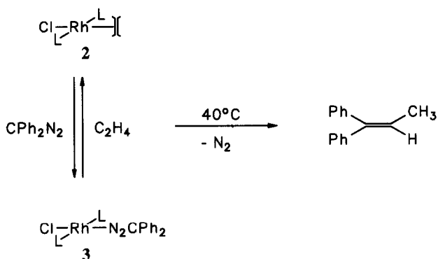
Scheme 1. Catalytic formation of 1,1-diphenylpropene ( \text{L} = \text{P}^i\text{Pr}_3 ).
